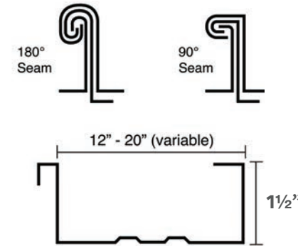
Panel (ribs & striations optional)
