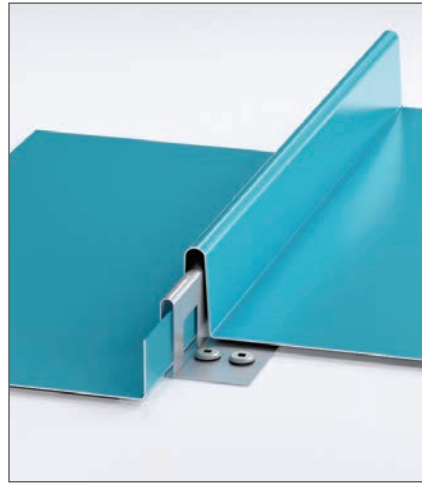
A1000 1 1/2" Snap-Lock Panel
