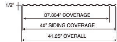
2.67" x .5" Corrugated Wall Panel System
