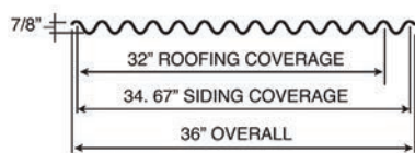
2.67" x .875" Corrugated Wall Panel System
