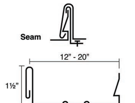
Panel (ribs optional)
