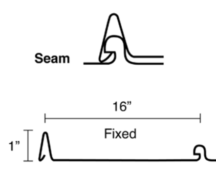
Panel (ribs & striations optional)
