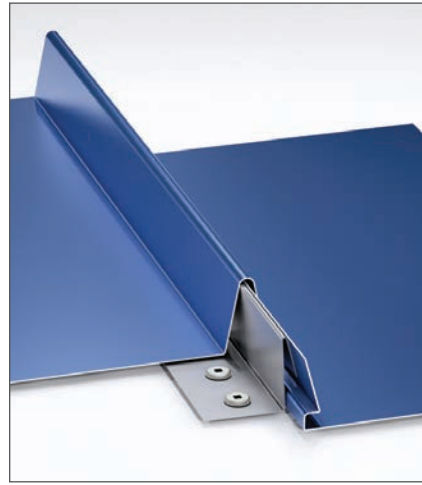
A1100 1 1/4" Integral Snap-Lock Panel
