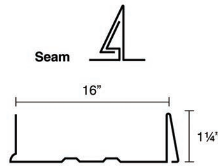
Panel (ribs optional)
