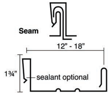
Panel (ribs & snap-on batten optional)
