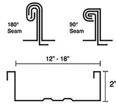
Panel (ribs optional)
