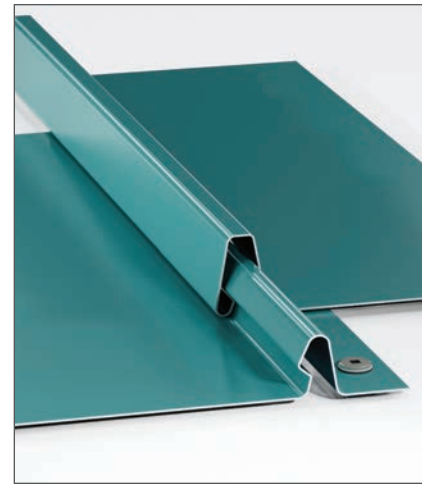
A1101/A1120 1" Integral Snap-Lock
